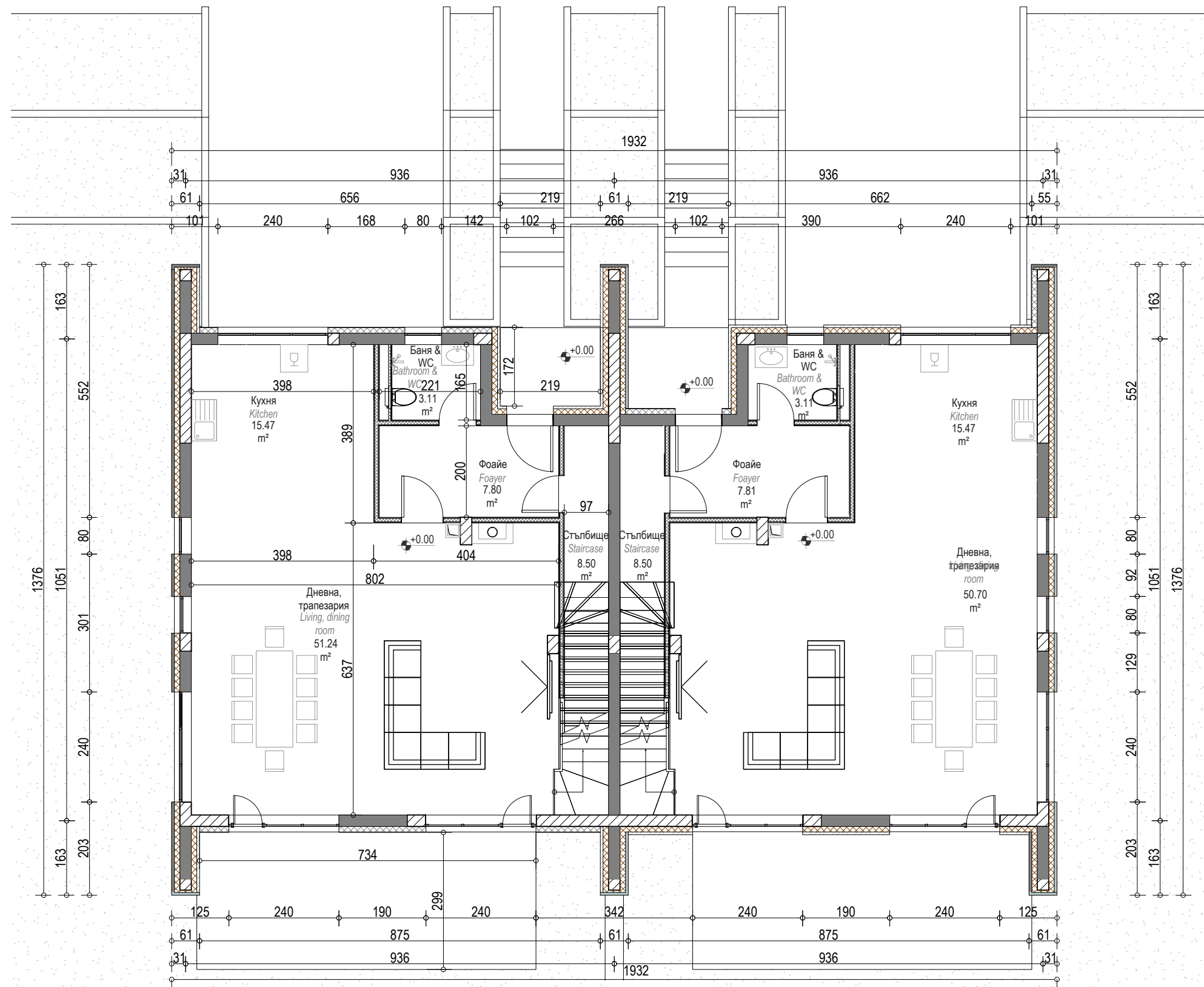
TWIN HOUSE TYPE A - Ground floor
