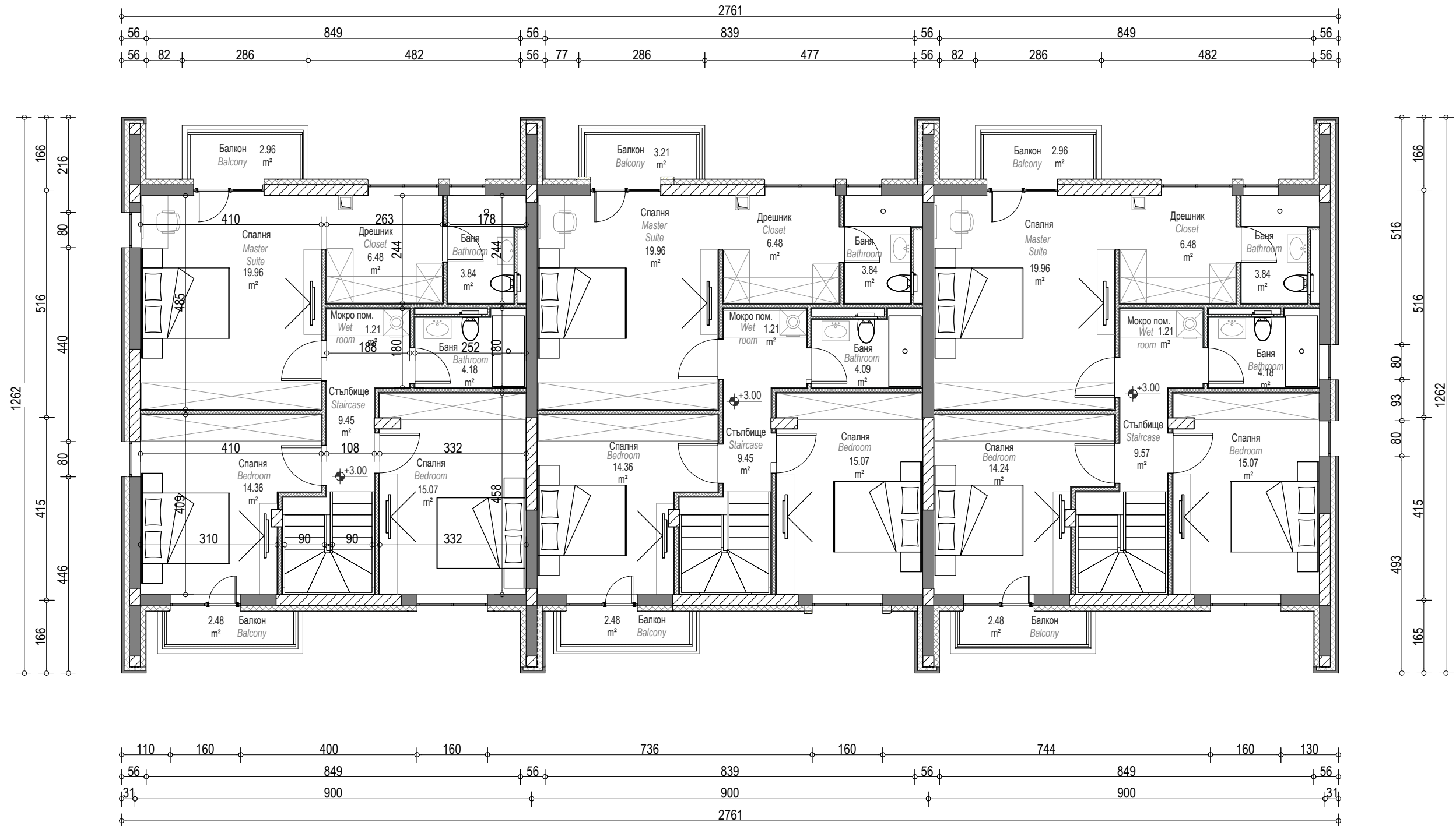
ROW HOUSE TYPE A - First floor
