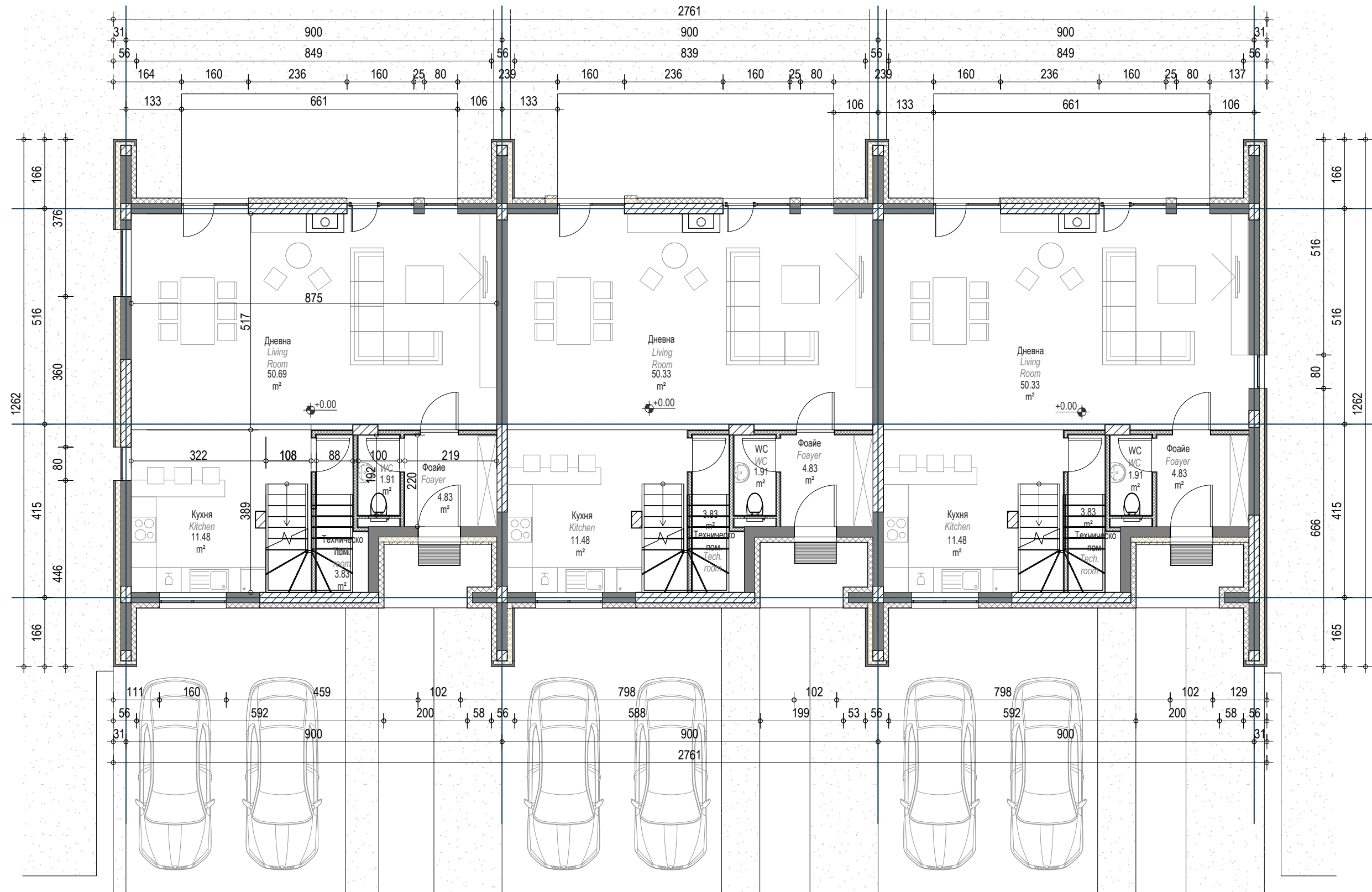
ROW HOUSE TYPE A - Ground floor
